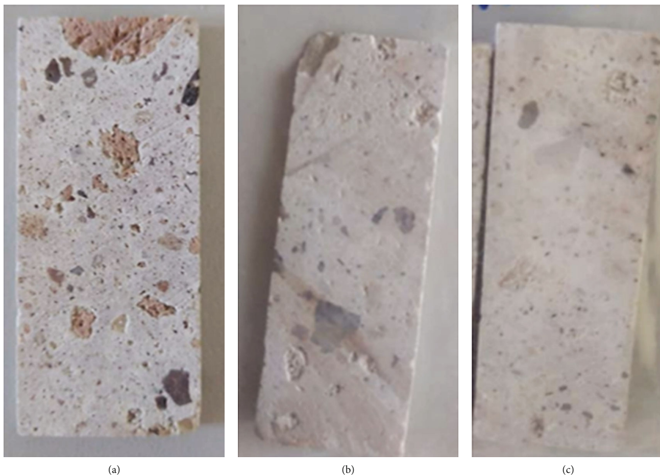
FIGURE 1: Photographs of (a) ignimbrite, (b) 10TEOS-5TiO 2 , and (c) 15TEOS-5TiO 2 samples.
