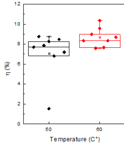
Figure 4. Efficiencies with preheating at 50 °C and 60 °C.
