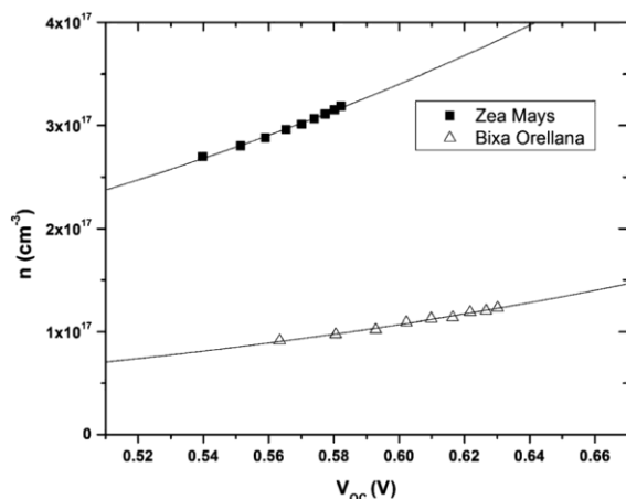
Fig. 9 Electronic density extracted as a function of open circuit voltage with its corresponding adjustment curves according to eqn (3).
