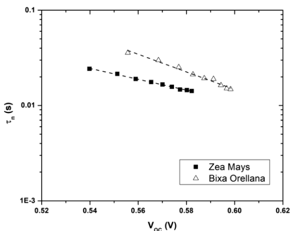
Fig. 7 Electron life time ( s_n ) as a function of the open circuit potential for devices manufactured with Zea mays and Bixa orellana .
