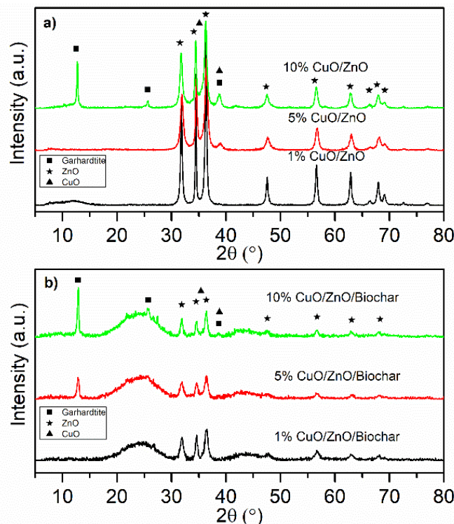
Figure 1. The XRD diffractograms of a) \text{CuO}/\text{ZnO} oxides and b) \text{CuO}/\text{ZnO}/\text{Biochars} .
