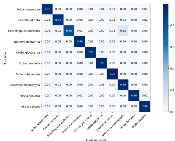
(a) Confusion matrix of the VGG-19 architecture for the raw testing set.
