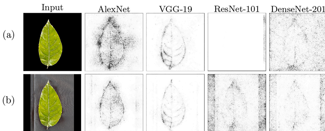
Fig. 7. Feature visualization of the models (trained with raw images) given a (a) raw input, or a (b) pre-processed input.
